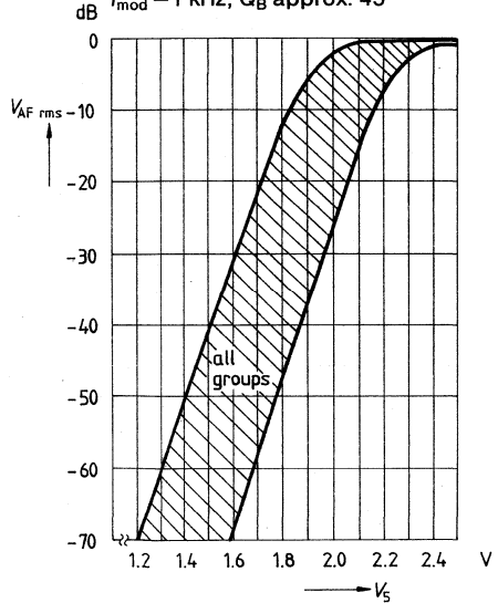
Volume control versus voltage to pin 5 V_S = 12\text{ V} ; f_z = 5.5\text{ MHz} ; \Delta f = \pm 50\text{ kHz} f_{\text{mod}} = 1\text{ kHz} ; Q_B \text{ approx. } 45
