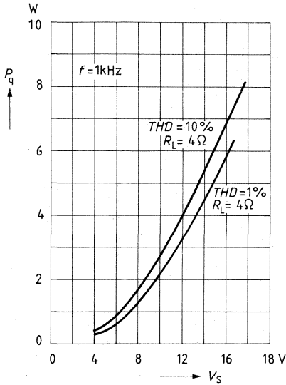
Stereo operation Output power versus supply voltage
