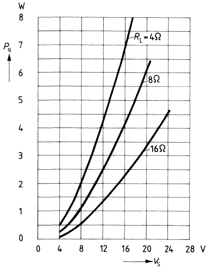
Output power versus supply voltage THD = 10%; R_L = 4, 8, 16 \Omega ; f = 1 \text{ kHz}
