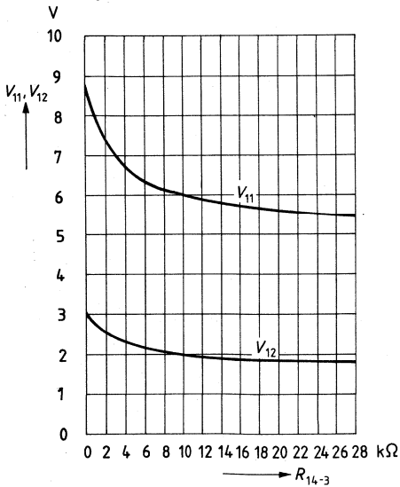
DC output voltage versus white level resistance
