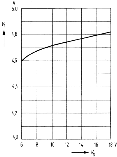
Z voltage versus supply voltage
