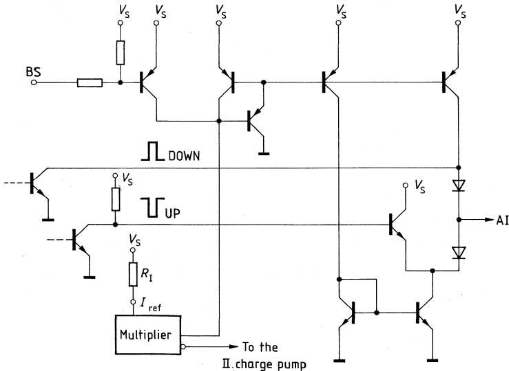
Charge pump
