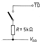
Connection of the \overline{\text{TD}} -input
