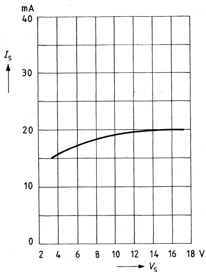
Quiescent current versus supply voltage
