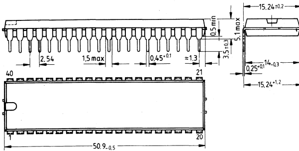
Plastic plug-in package 20 B 40 DIN 41 866, 40 pins, DIP
