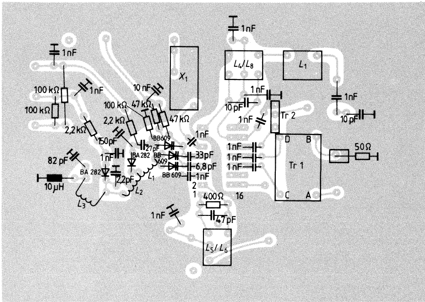
PCB layout of test and measurement circuit 1
