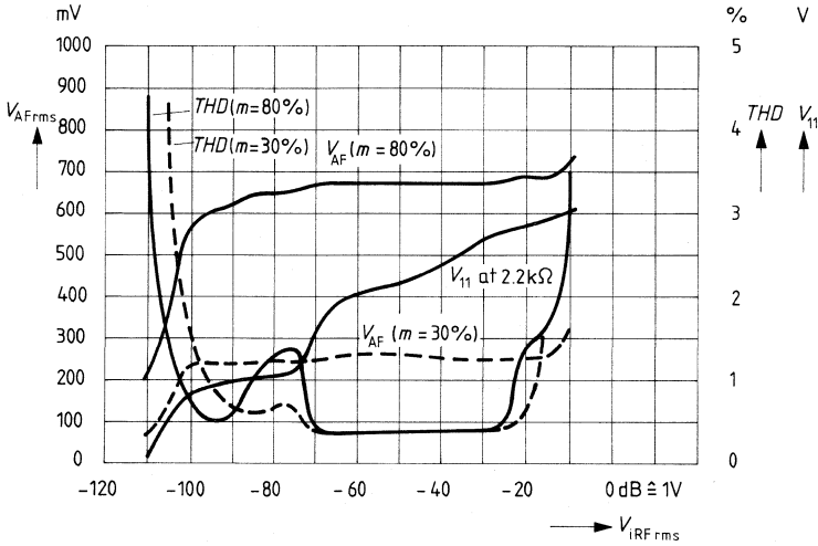
AF output voltage, total harmonic distortion, instrument voltage versus RF input voltage V_S = 15\text{ V} , f_{RF} = 1000\text{ kHz} , f_{mod} = 1\text{ kHz} Coupling with wideband circuit
