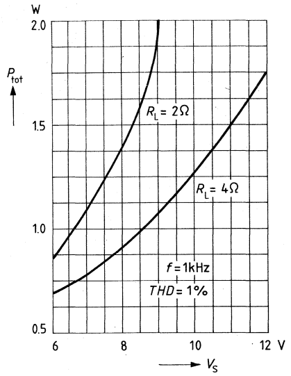
Total power dissipation versus supply voltage
