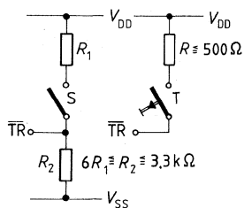
Connection of the \overline{\text{TR}} input
