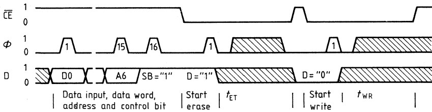
Figure 2: Reprogramming cycle (1 Kbit E 2 PROM)
