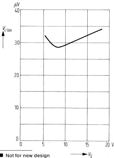
Input voltage for limiting versus supply voltage
