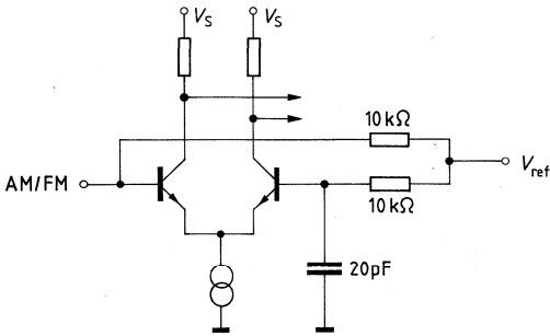
AM/FM inputs
