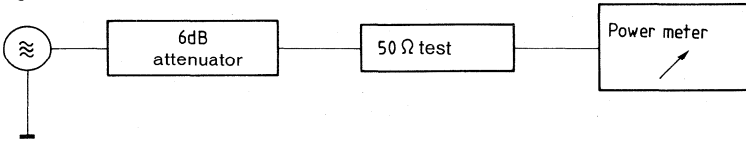
Test circuit 1: Calibration of the signal generator
