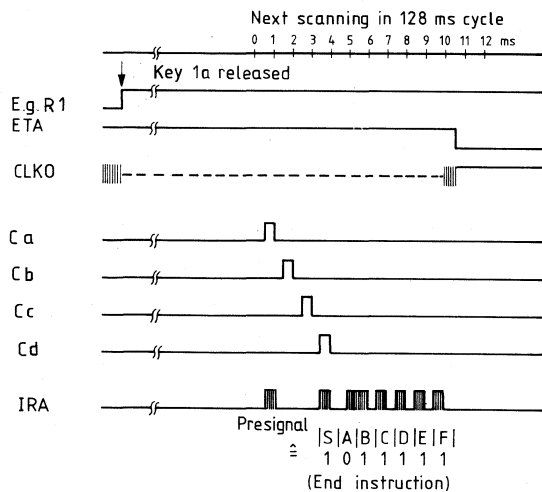
Timing diagram 3 (releasing a key)
