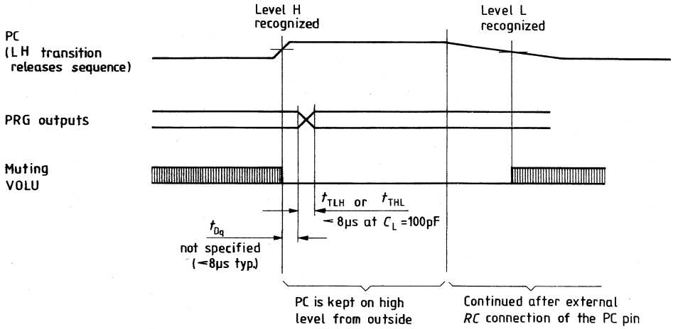
Timing diagram 3
