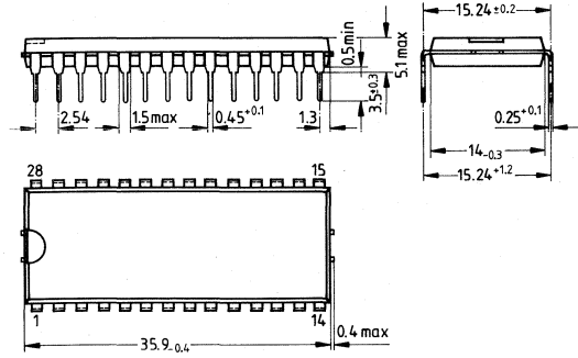
Plastic plug-in package 20 B 28 DIN 41 866, 28 pins, DIP
