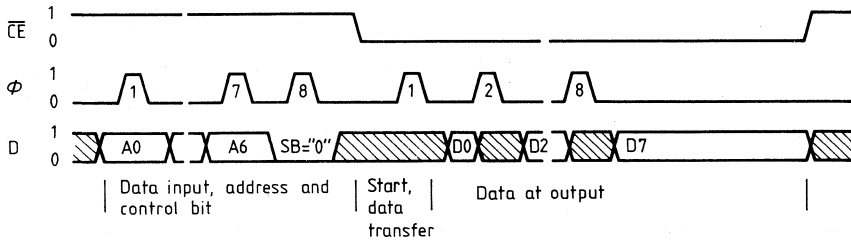
Figure 1: Read cycle (1 Kbit E 2 PROM)
