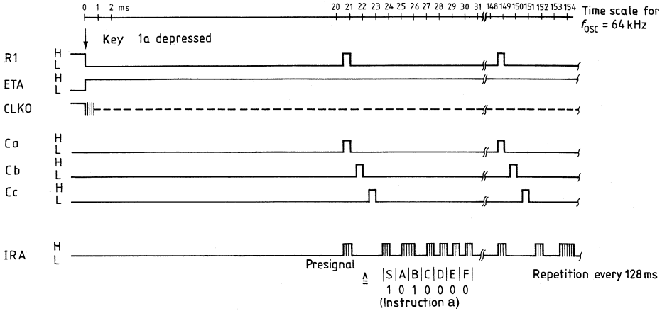
Timing diagram 2 (pressing a key)
