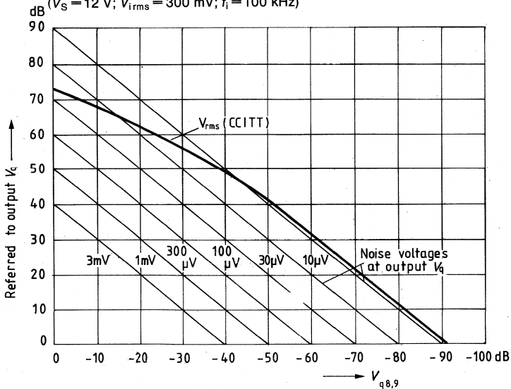
Disturbance voltage spacing versus attenuation ( V_S = 12\text{ V} ; V_{i,rms} = 300\text{ mV} ; f_i = 100\text{ kHz} )
