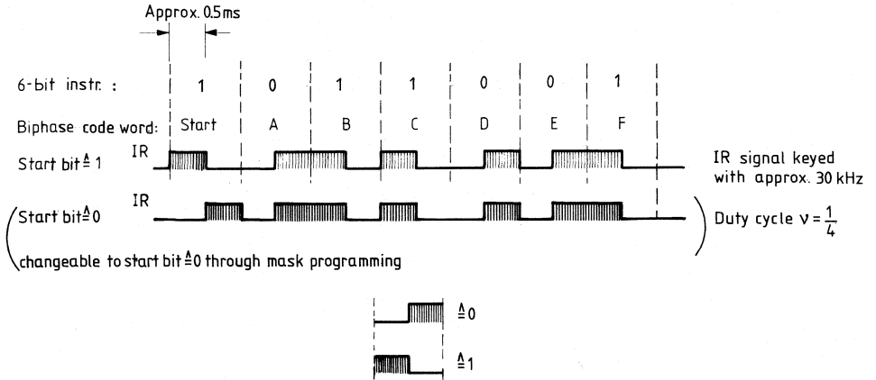
Timing diagram 1 (biphase coding, plotted without presignal)
